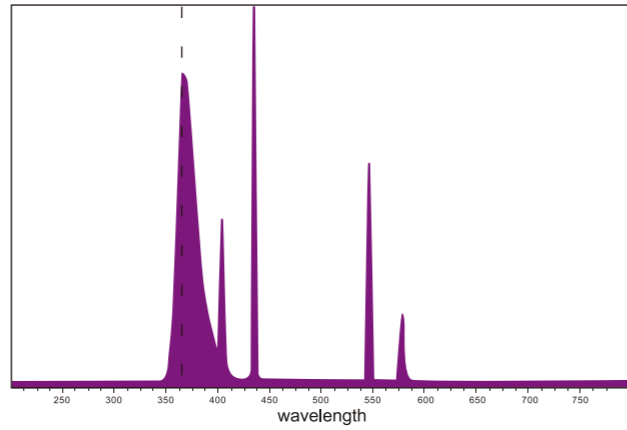
UVA CFL White light tube Spectrum
