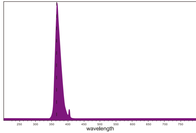
UVA CFL Black light tube Spectrum
